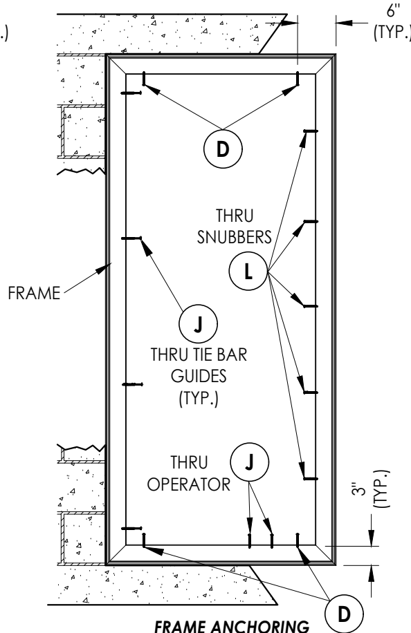
FRAME ANCHORING Direct to Masonry
