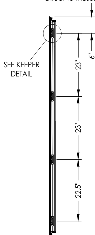
KEEPER LOCATIONS 4 Total
