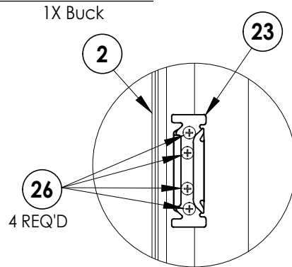
KEEPER DETAIL
