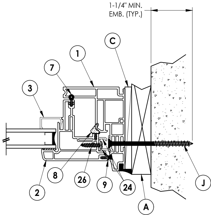
1 3 HORIZONTAL CROSS SECTION Shown w/ 1X Buck
