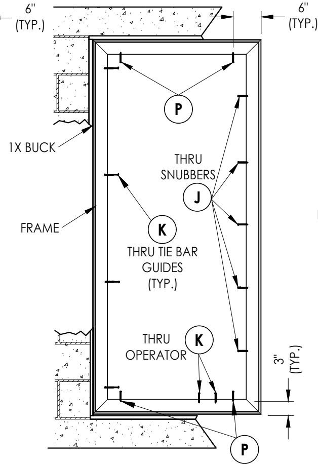
FRAME ANCHORING 1X Buck
