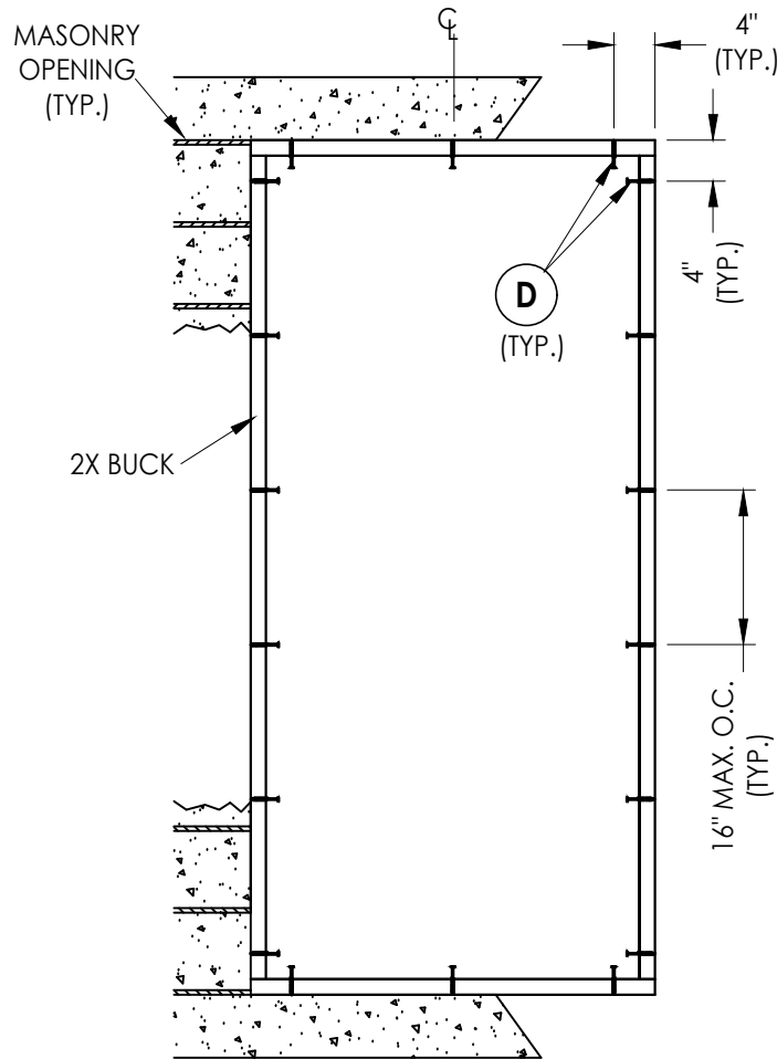
BUCK ANCHORING
