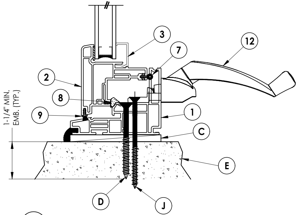
2 3 VERTICAL CROSS SECTION Shown w/ 1X Buck @ head & Direct to Masonry @ sill
