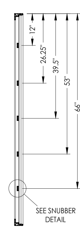
SNUBBER LOCATIONS 5 Total
