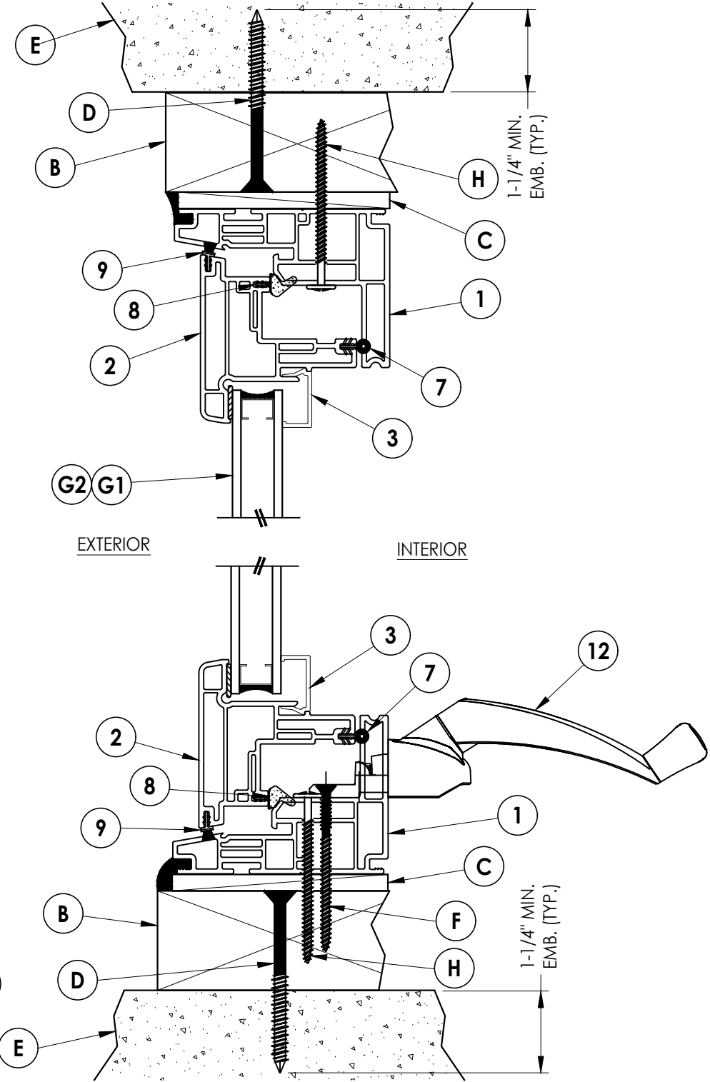
2 VERTICAL CROSS SECTION Shown w/ 2X Buck
