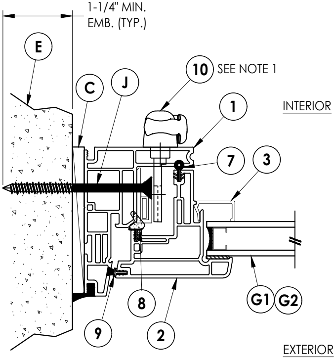
3 HORIZONTAL CROSS SECTION Shown Direct to Masonry
