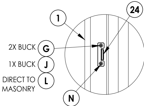
SNUBBER DETAIL
