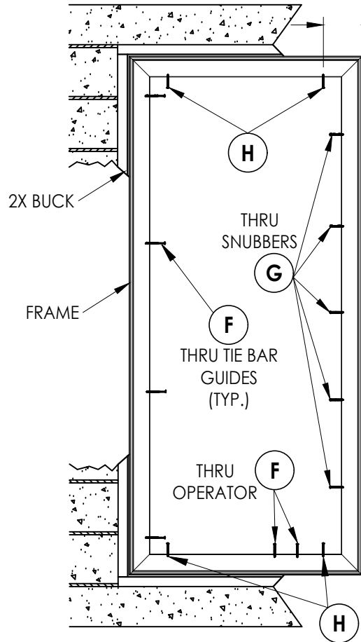
FRAME ANCHORING 2X Buck
