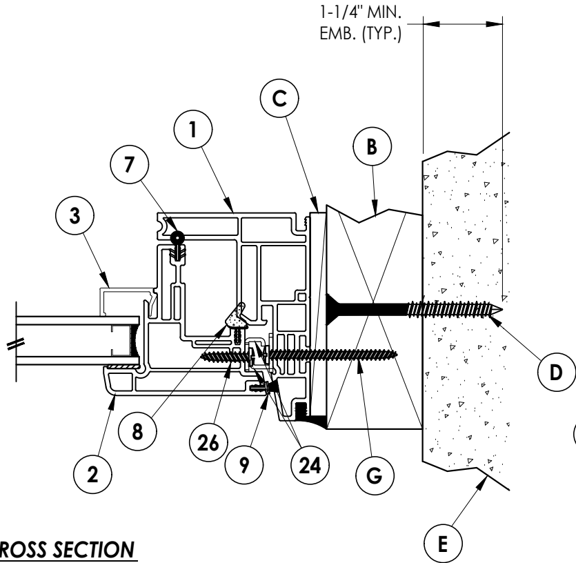
3 HORIZONTAL CROSS SECTION Shown Direct to Masonry
